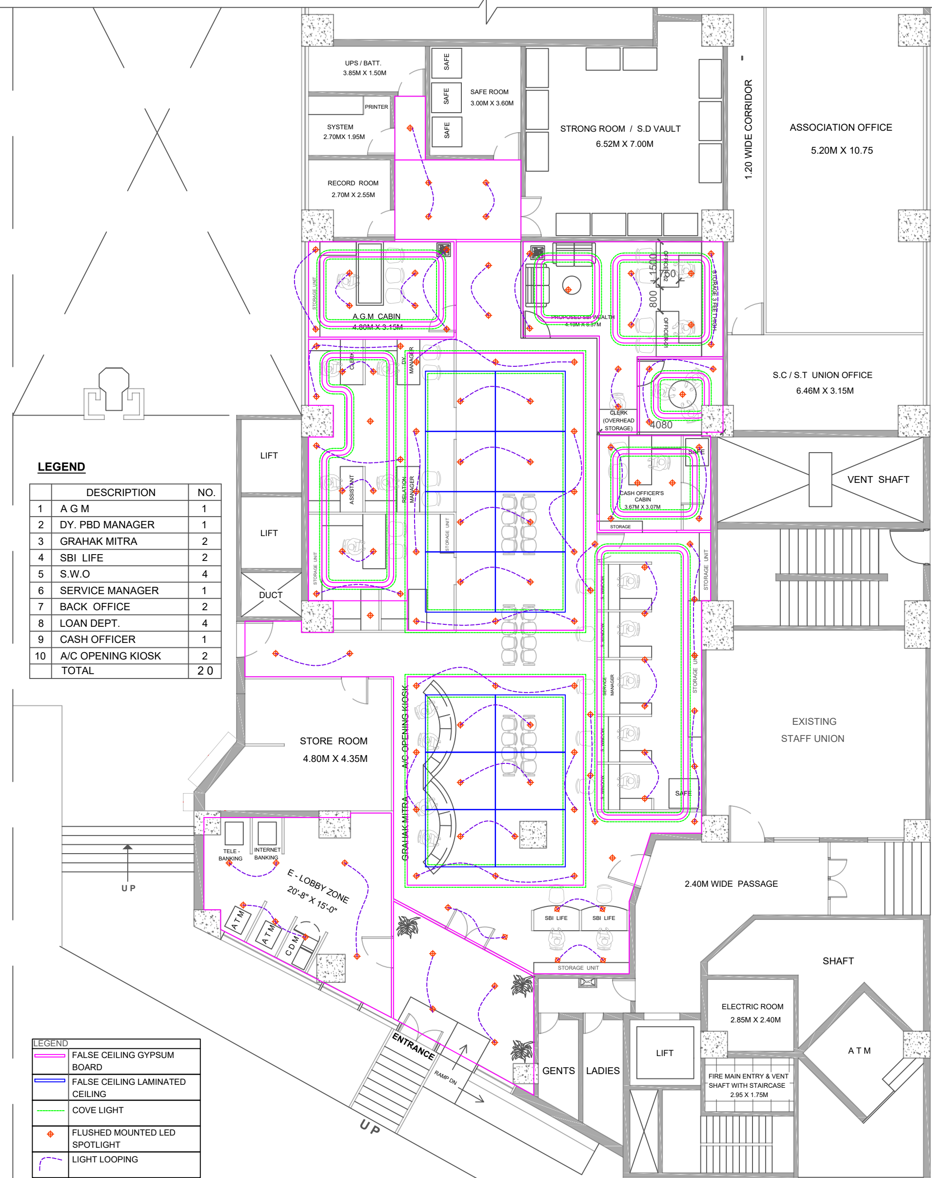
FALSE CEILING LAYOUT
